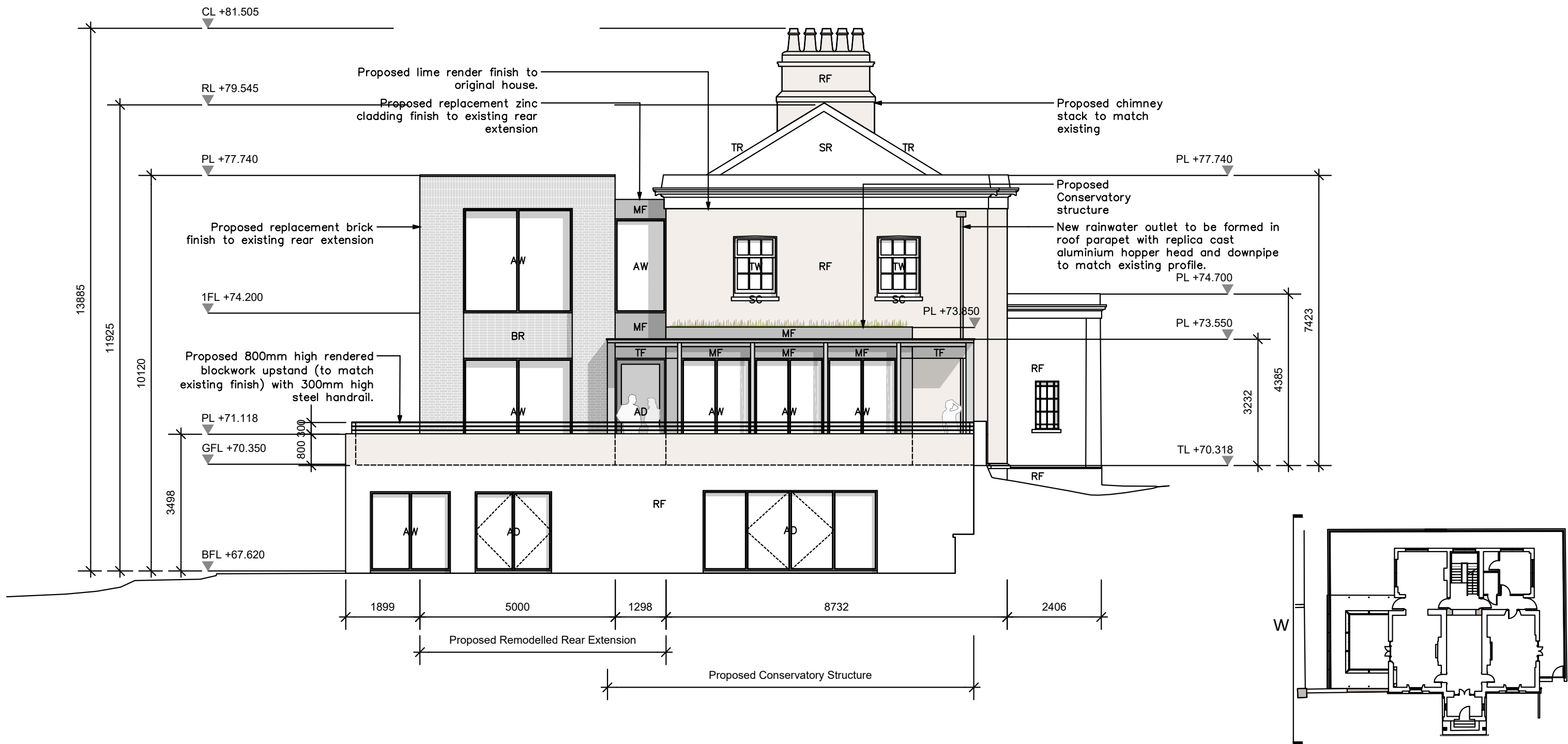
Cedar Mount House, Proposed West Elevation
